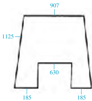
23/4000-84 (D9035, 5136368) Parabrisas Windscreen
